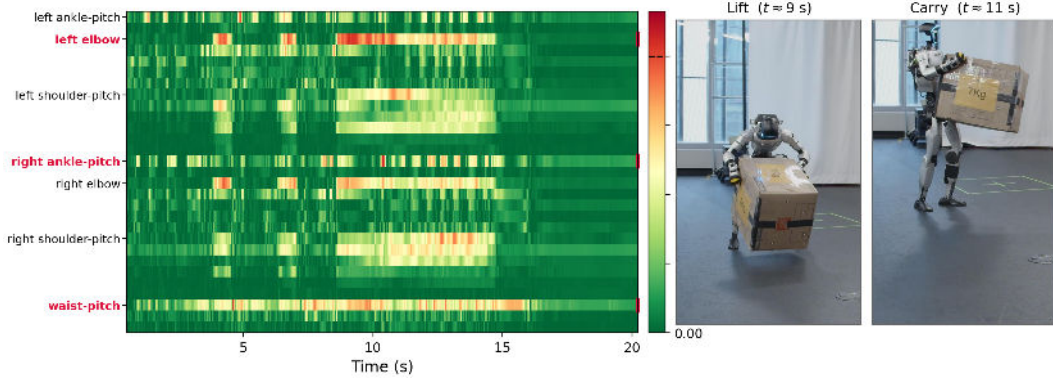
Figure 2: Per-joint torque during the 7 kg experiment, normalized by each joint’s effort limit (only discussed joints labeled; over-limit in bold red, dashed line marks 100 %). Snapshots: lift ( t \approx 9 s) and carry ( t \approx 11 s).
