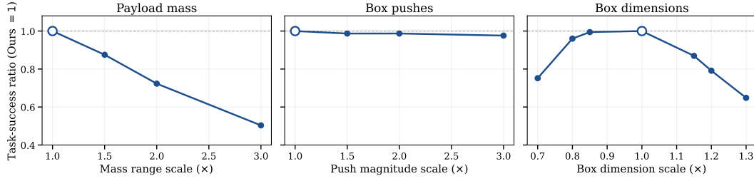
Figure 3: Robustness Study (20 s). Task-success ratio (Ours nominal = 1) under 3 perturbation axes (box mass, external pushes, box dimensions) scaled relative to the training distribution.
