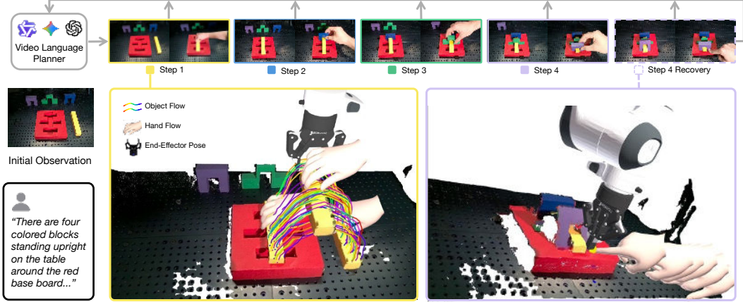
Figure 1: Zero-shot long-horizon manipulation with NovaPlan. Given a task command and an initial observation, a video language planner is used to select and generate the best next-step video. Executable robot actions are extracted from the video through object or hand flow tracking. The updated observation is sent back to the planner to enable closed-loop reasoning and recovery from failure states.
