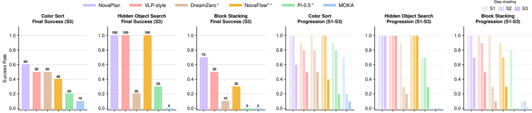
Figure 5: Long-horizon task performance. (Left) Final success rate of different methods on three long-horizon tasks. (Right) Success rate of each method after every step of the three long-horizon tasks, where shading denotes the step index. Methods marked with ^+ (NovaFlow, DreamZero, and \pi_{0.5} ) receive oracle high-level plans; MOKA and VLP-style generate their own plans.
