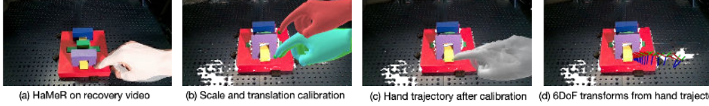
Figure 3: Geometric grounding for non-prehensile recovery. (a) HaMeR [46] predicts the MANO hand mesh on the generated recovery video. (b) Red: mesh from raw prediction. Green: mesh after scale calibration. Cyan: mesh after additional translation offset enforcing fingertip and object surface contact. (c) The hand trajectory after calibration. (d) Calibrated trajectory converted into per-frame SE(3) transforms.
