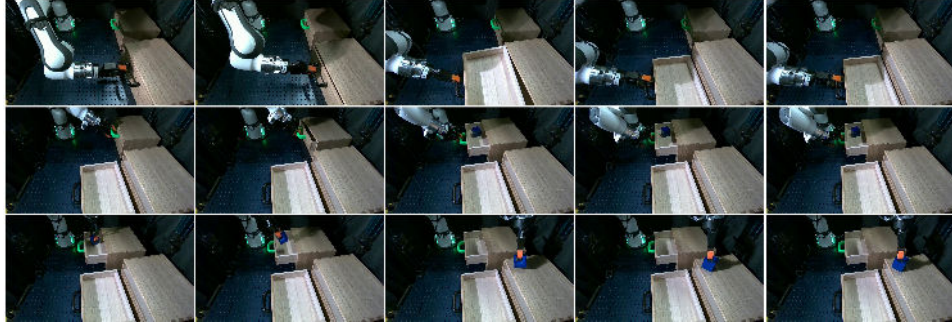
Figure 13: Hidden object search experiment. Each row in this figure illustrates a distinct, sequential step in the hidden object search task. The frames in each row display the execution of that specific step, ordered chronologically from left to right. This rollout shows an example of planning under partial observability where the robot must open drawers to reveal the target object.
