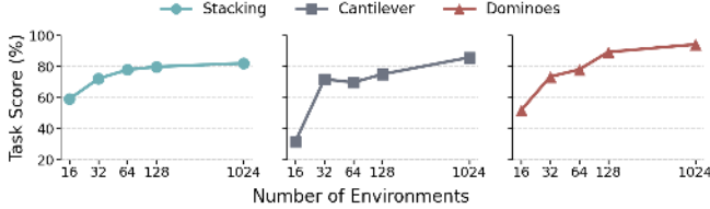
Fig. 7. Effect of simulation parallelism on task score. More environments improve performance on all tasks, showing that Simify benefits from additional test-time compute.
